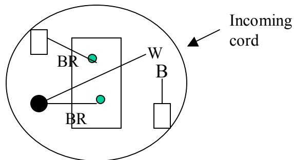
Single Speed Switch
