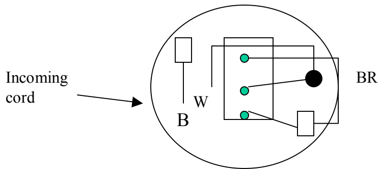
Two Speed Switch
